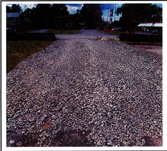
Construction entrance installed.
