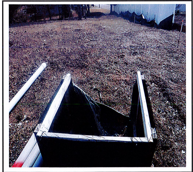
CB 2 drop inlet protection requires repair.
