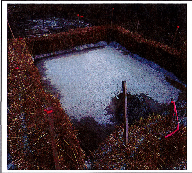
Concrete washout needs to be replaced before the next concrete pour. It is past 50% capacity.
