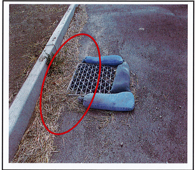
Inlet protection placed is not protecting the catch basin. More bags are needed.
