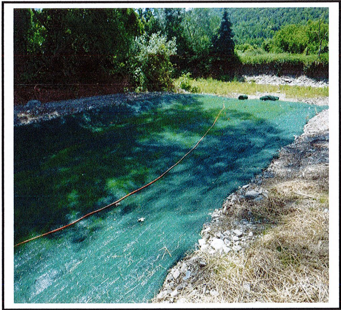
Infiltration basin emergency spillway.
