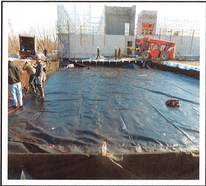
Underground Detention #1- Welding membrane.
